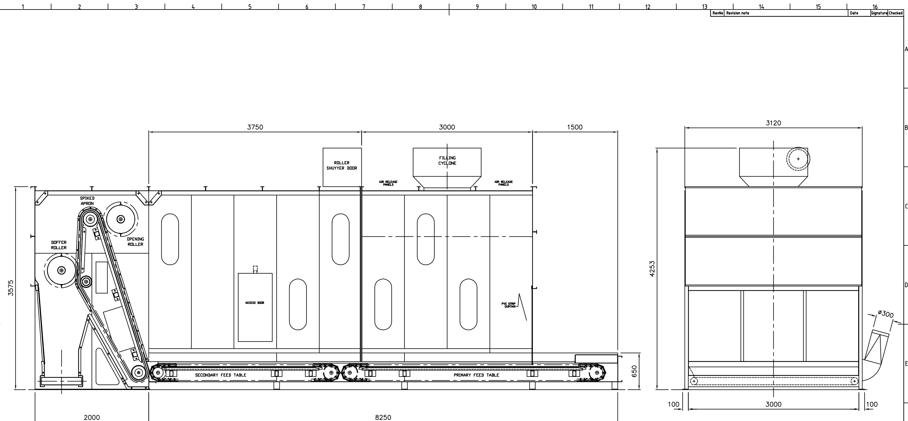
SECTIONAL SIDE ELEVATION
