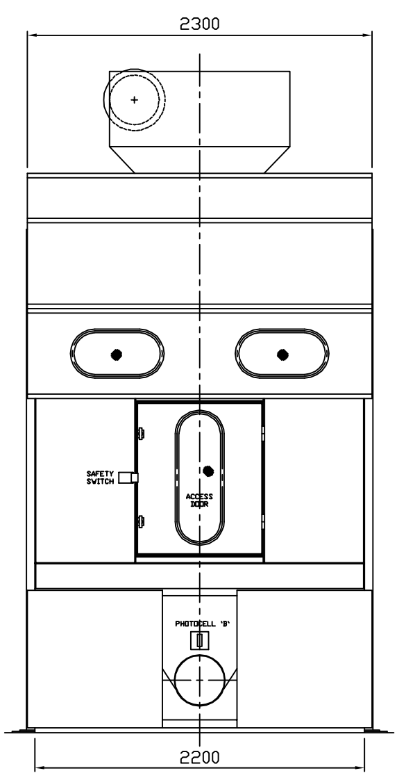
END ELEVATION ON FRONT OF EMPTYING HEAD
