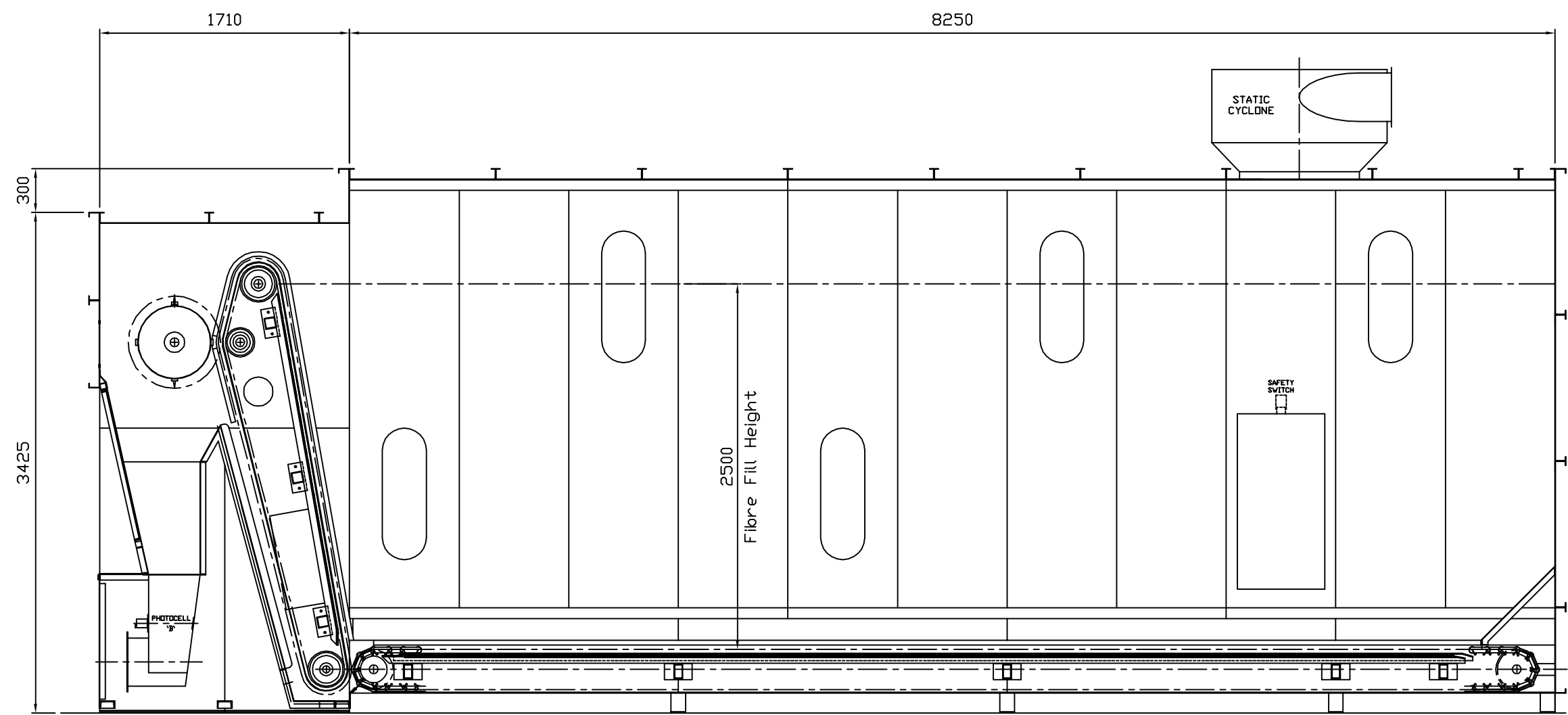
SECTIONAL SIDE ELEVATION
