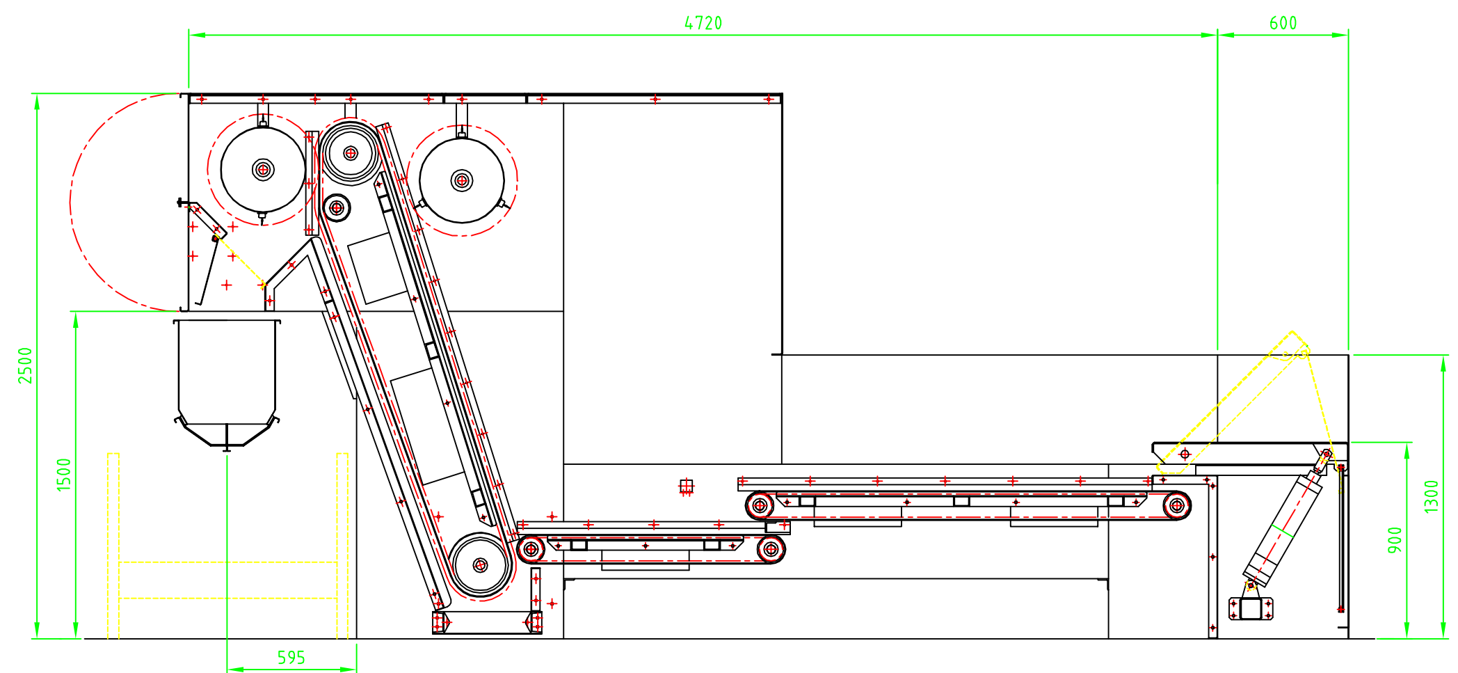
SECTIONAL SIDE ELEVATION
